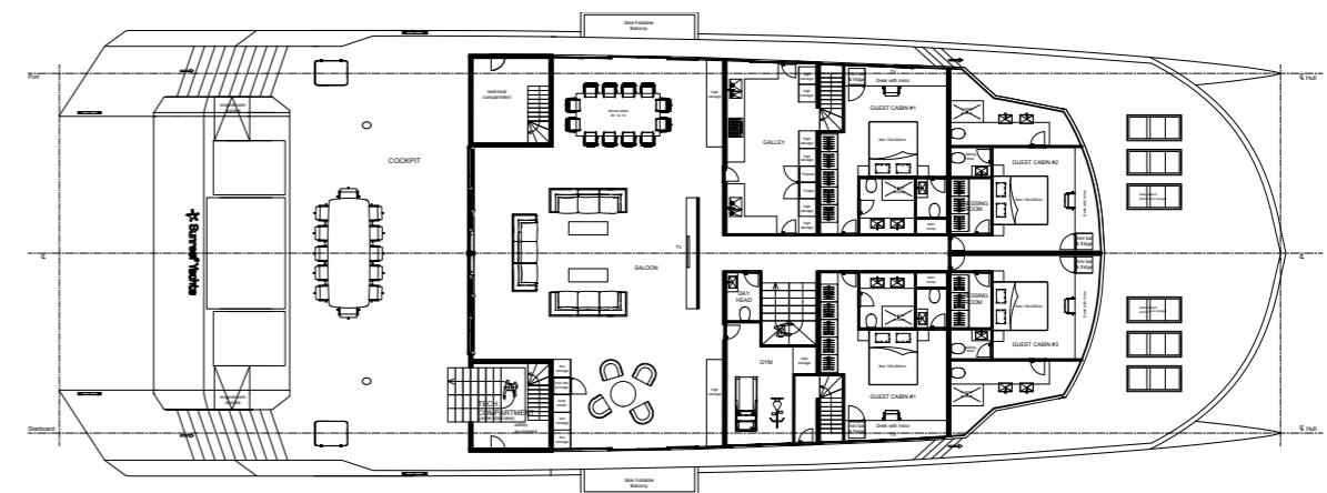
MAIN DECK
