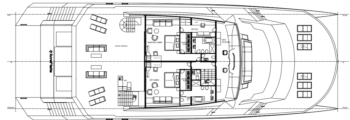
UPPER DECK
